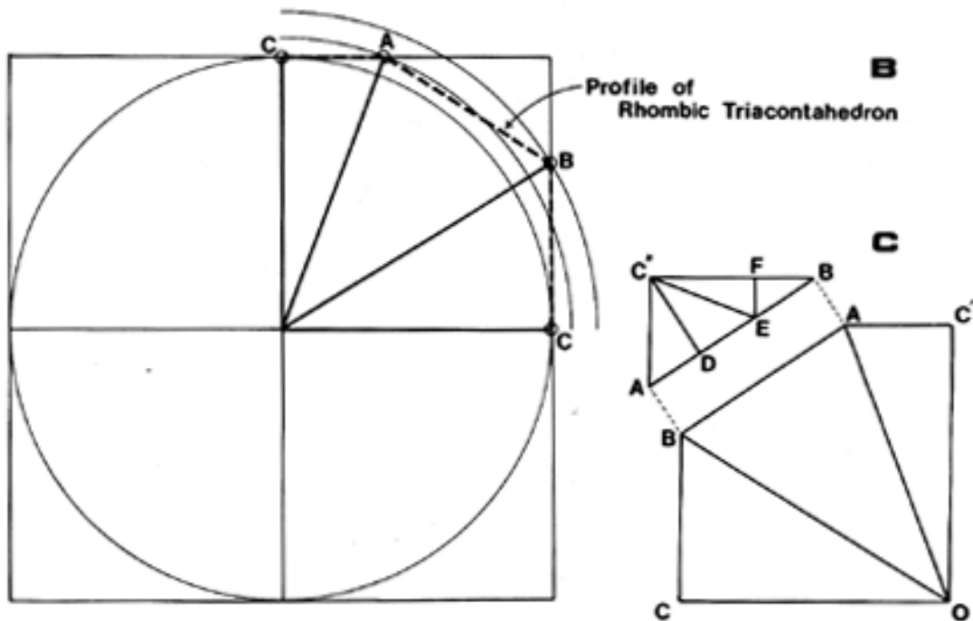
Fig. 986.508 Six Intertangent Great-circle Discs: Twelve-inch module grids divided into 24 quadrant blanks at A Profile of rhombic triacontahedron superimposed on quadrant at B.
